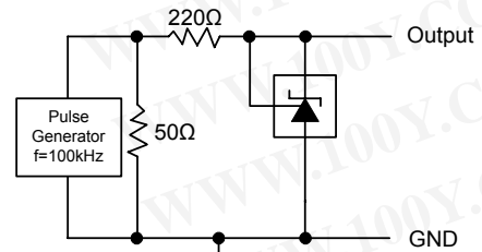
TEST CIRCUIT FOR PULSE RESPONSE
