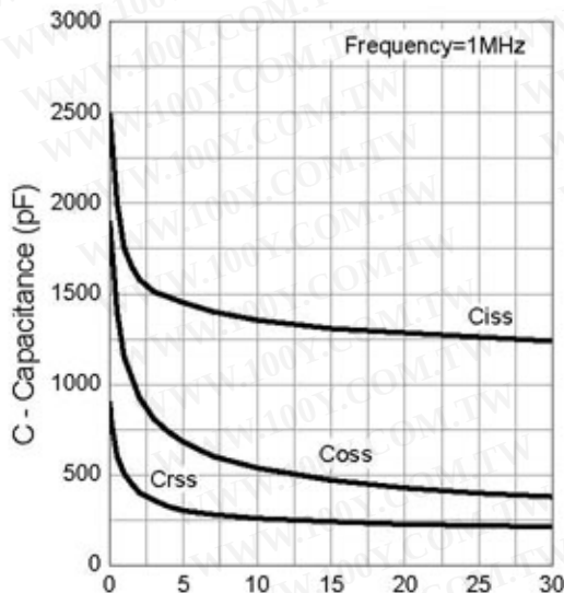
Capacitance
