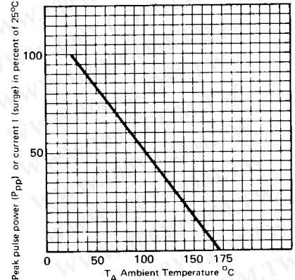
FIG. 3. Derating curve
