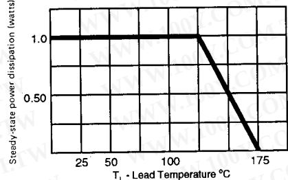
FIG. 4. Steady-state power derating curve
