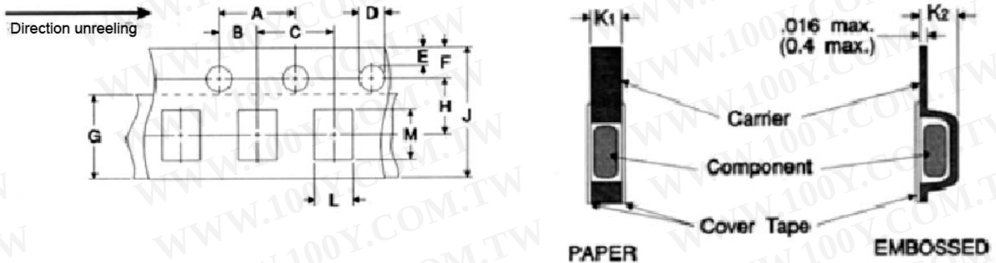
Packaging (0603, 0805, 1206, 1210, 2010, 2512)
