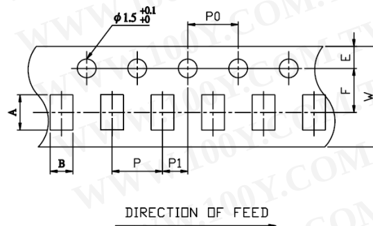
TE CARRIER TAPE
