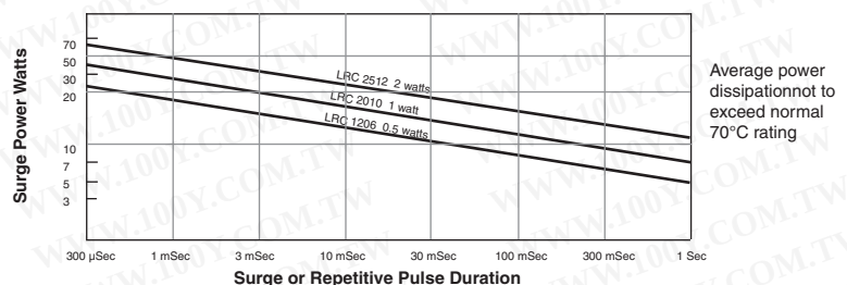
Pulse and Surge Capability
