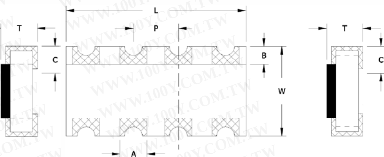
Package Drawing – Concave, Type C
