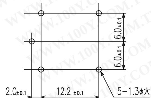
4. DRILLING DIAGRAM(BOTTOM VIEW)
