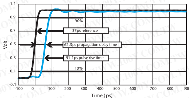
RF300/RF303 Time Response (RF Note 6)
