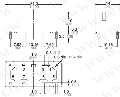
External dimensions
