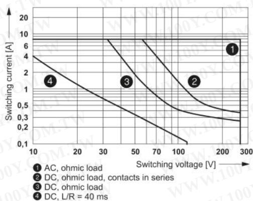
Interrupting rating
