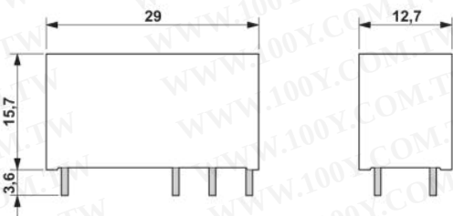
Dimensioned drawing
