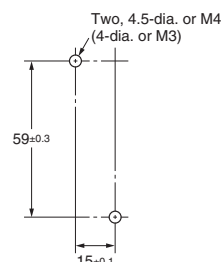
Mounting Hole Dimensions (Top View)
