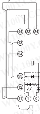
G7SA-3A1B Mounted
