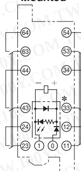
G7SA-5A1B Mounted
