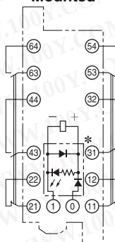
G7SA-3A3B Mounted
