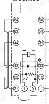
G7SA-4A2B Mounted
