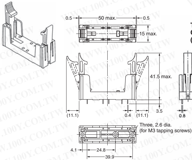
G7SA-3A1B Mounted
