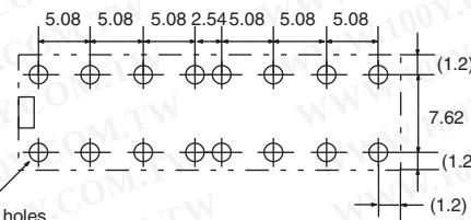
Mounting Holes (Bottom View) Tolerance: \pm 0.1
