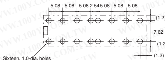
Mounting Holes (Bottom View) Tolerance: \pm 0.1
