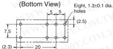
Mounting Holes (Bottom View)
