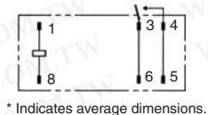
Terminal Arrangement/ Internal Connection (Bottom View)
