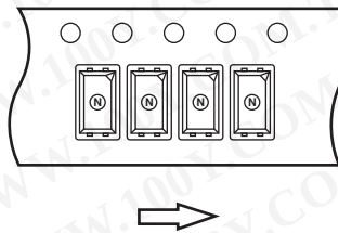
Outline and Dimensions (Reel)
