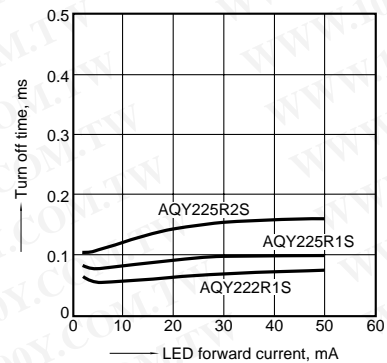
11. Turn off time vs. LED forward current characteristics Measured portion: between terminals 3 and 4 Load voltage: 10V (DC) Continuous load current: 100mA (DC) Ambient temperature: 25°C 77°F
