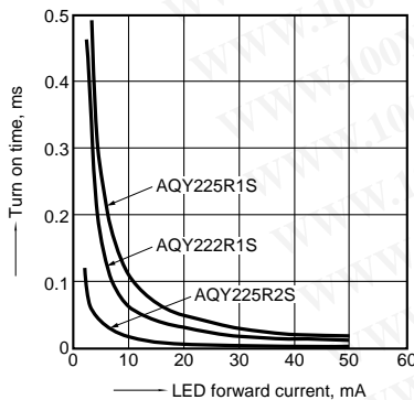
10. Turn on time vs. LED forward current characteristics Measured portion: between terminals 3 and 4 Load voltage: 10V (DC) Continuous load current: 100mA (DC) Ambient temperature: 25°C 77°F
