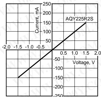
8.-(3) Current vs. voltage characteristics of output at MOS portion Measured portion: between terminals 3 and 4 Ambient temperature: 25°C 77°F
