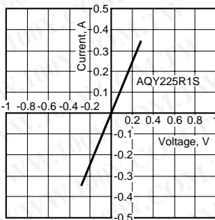
8.-(2) Current vs. voltage characteristics of output at MOS portion Measured portion: between terminals 3 and 4 Ambient temperature: 25°C 77°F
