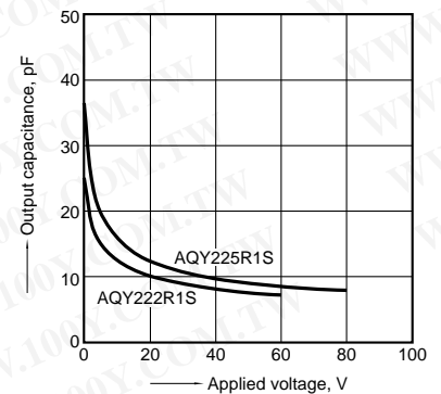
12.-(1) Output capacitance vs. applied voltage characteristics Measured portion: between terminals 3 and 4 Frequency: 1 MHz, 30m Vrms Ambient temperature: 25°C 77°F
