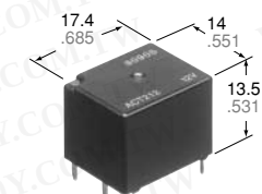
Twin type (8 terminals)
