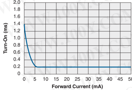
Typical Turn-On vs. LED Forward Current ( I_L=1\text{A}_{DC} )
