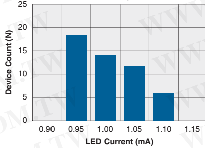
Typical I_F for Switch Operation (N=50, I_L=1\text{A}_{DC} , T_A=25^\circ\text{C} )
