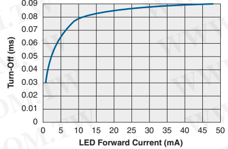
Typical Turn-Off vs. LED Forward Current ( I_L=1\text{A}_{DC} )
