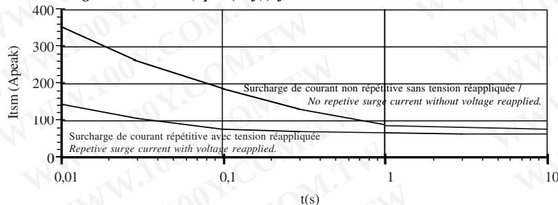
Fig.3 Surchage de courant : I_{tsm} (A_{peak}) = f(t) pour modèle 40A ( I_{tsm}=350A ) Surge current : I_{tsm} (A_{peak}) = f(t) for 40A models with I_{tsm}=350A
