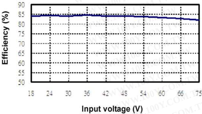
BUB15-48S1W Input voltage vs. Efficiency
