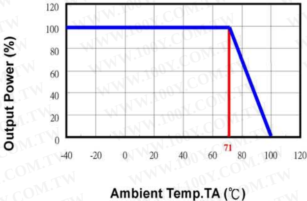
BUB15W Series Power Derating Curve(5)
