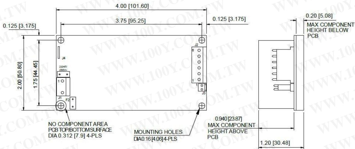
Figure 2 Dimension Drawing (Top and Side View)
