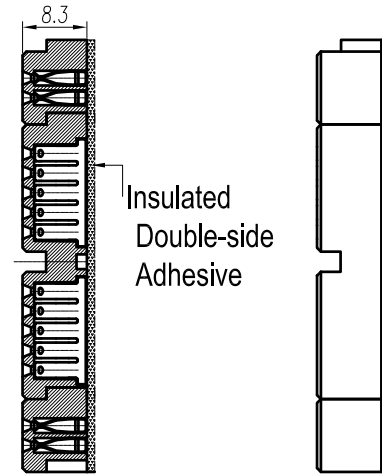
Section B-B
