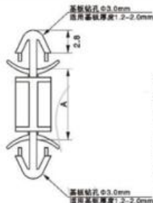
0306 PC板隔離柱 MINIATURE SUPPORT POST
