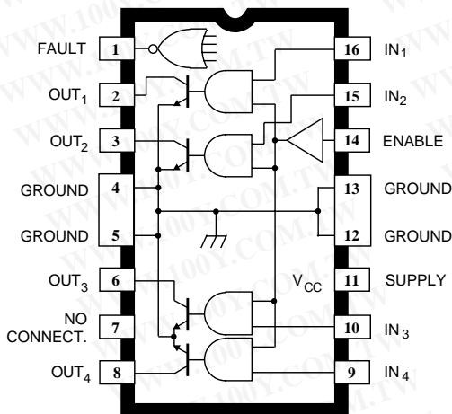
Dwg. PP-018A
