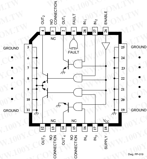
Dwg. PP-019
