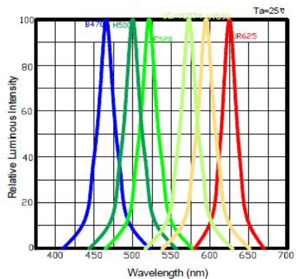
Wavelength Characteristics
