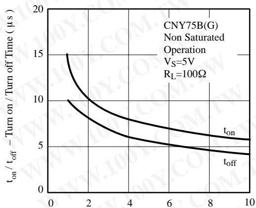
Figure 26. Turn on / off Time vs. Collector Current
