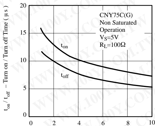
Figure 27. Turn on / off Time vs. Collector Current
