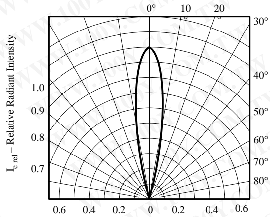
Figure 10. Relative Radiant Intensity vs. Angular Displacement
