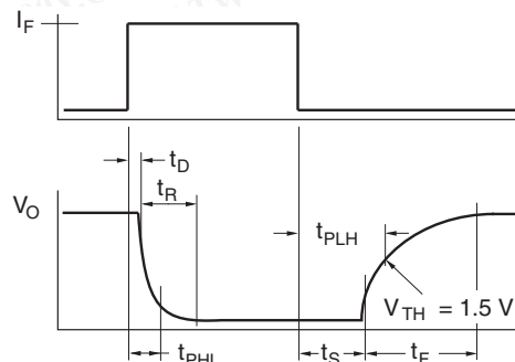
Fig. 8 - Switching Waveform
