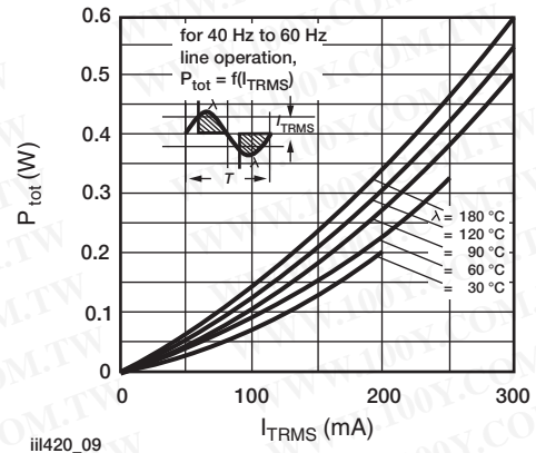
Fig. 9 - Power Dissipation
