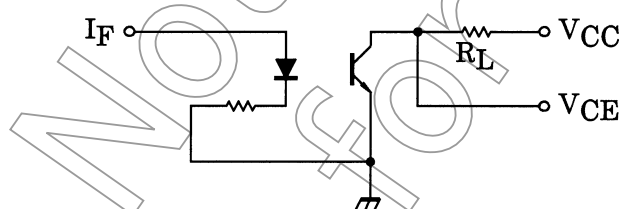
(Fig.1) Switching Time Test Circuit
