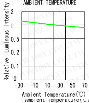
LUMINOUS INTENSITY VS. AMBIENT TEMPERATURE
