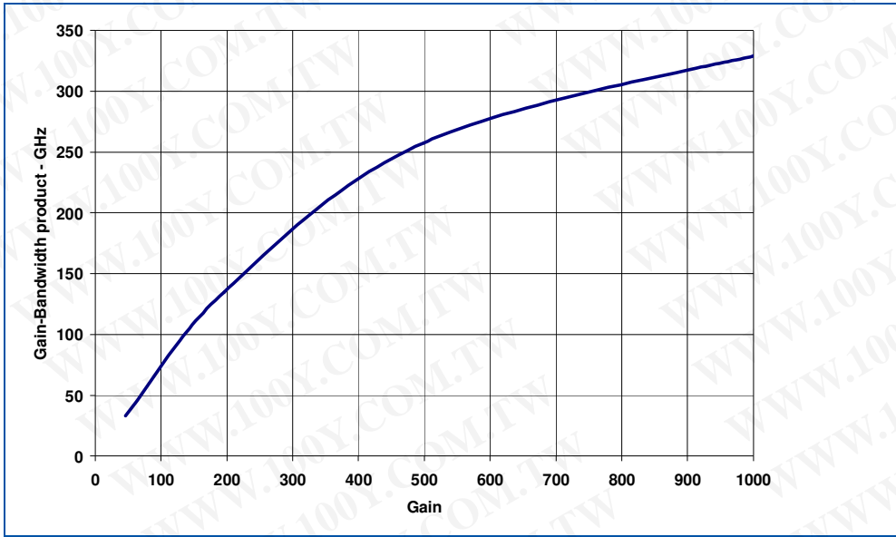
Figure 7 Typical Gain –bandwidth Product vs. Gain
