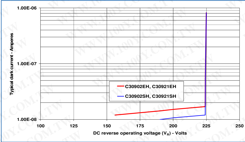
Figure 5 Typical dark current vs. operating voltage @ 22 °C
