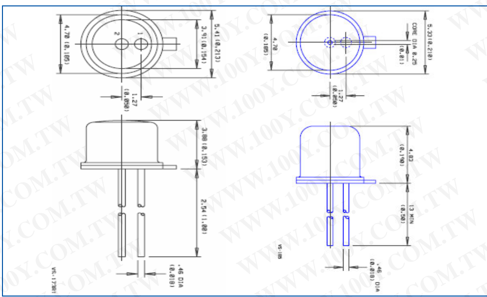
Figure 11 C30902SH (left) C30921SH (right) TO-18 Package outline
