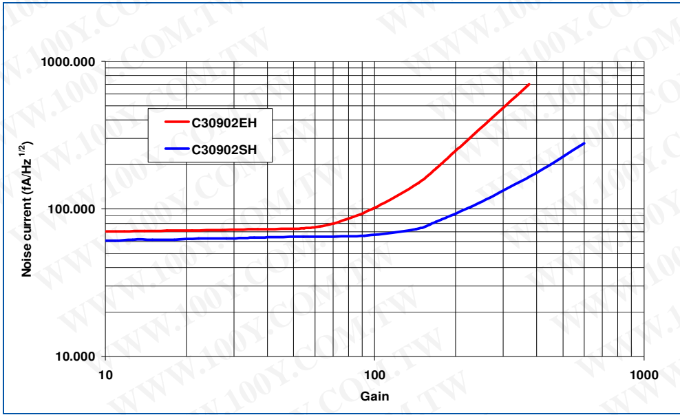
Figure 4 Typical Noise current vs. Gain
