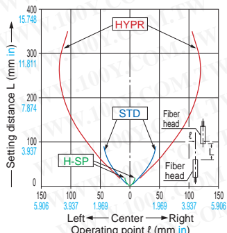
FT-S11 Thru-beam type
