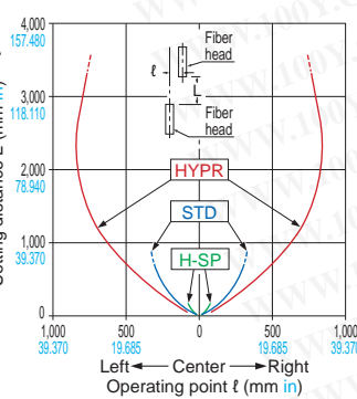
FT-H20-VJ50-S FT-H20-VJ80-S
