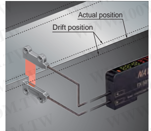
The drifting path can be monitored as the light intensity changes.
