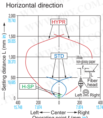
FD-60 Reflective type
