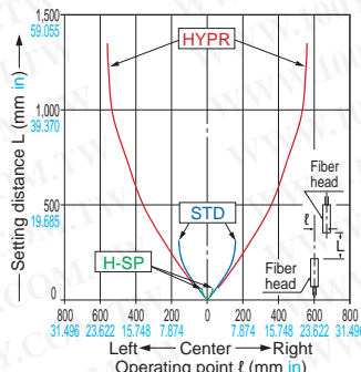
FT-S21 Thru-beam type
