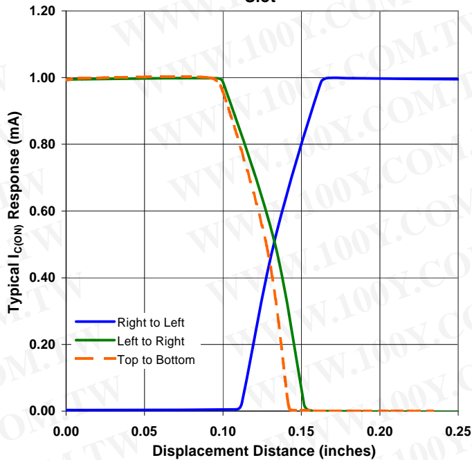
OPB827 thru OPB829 (A, C) - Flag in Middle of Slot
