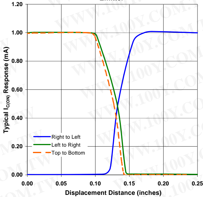
OPB827 thru OPB829 (A, C) - Flag Next to Emitter
