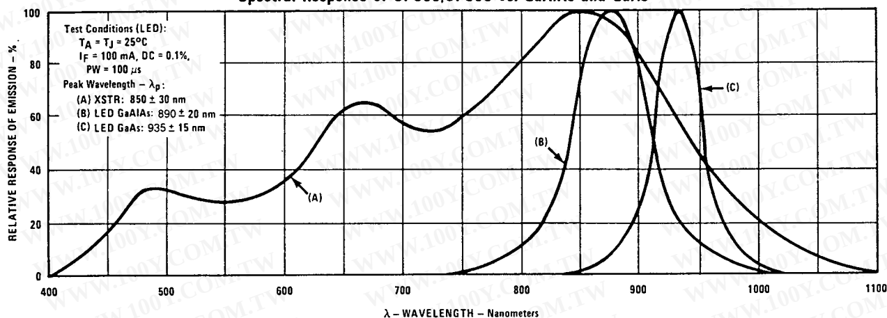
Spectral Response of OP593/OP598 vs. GaAlAs and GaAs
