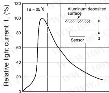
Sensing Distance Characteristics (Typical)
