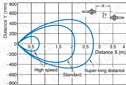
Through-beam E32-TC200
