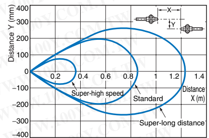
Through-beam E32-T22R
