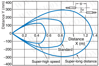
Through-beam E32-T11
