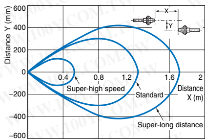
Through-beam E32-T12R
