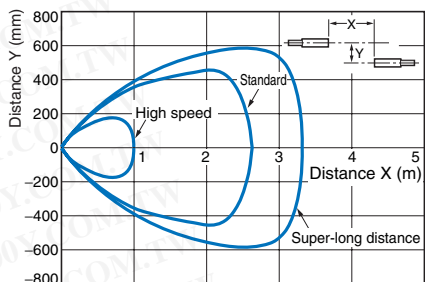
Through-beam E32-T11R
