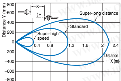
Through-beam E32-T11
