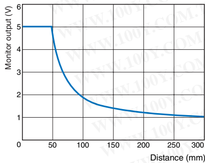
Through-beam E32-TC200
