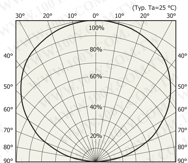
Relative sensitivity
