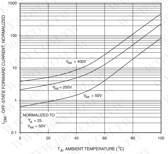
Figure 4. Off-State Current vs. Temperature
