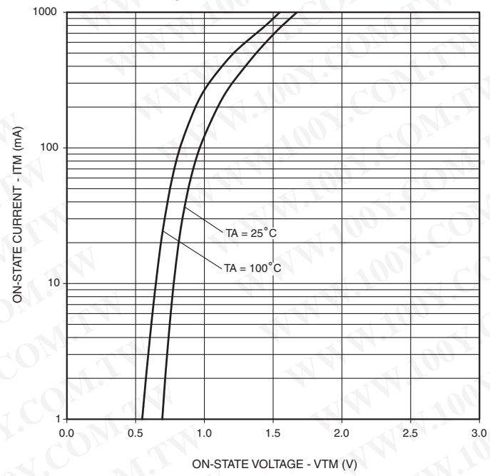
Figure 6. On-State Characteristics
