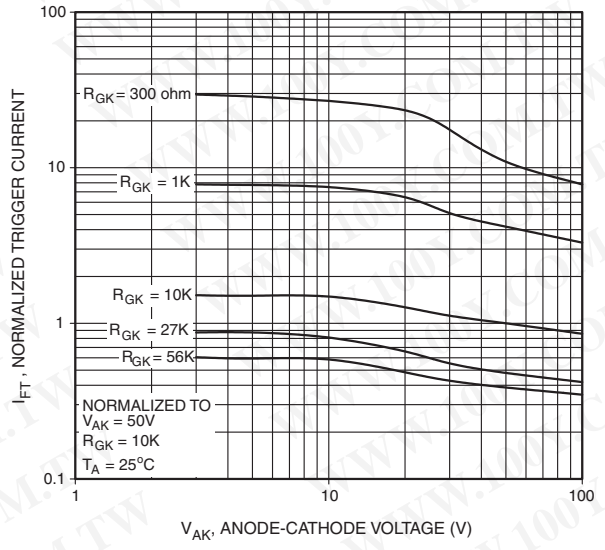
Figure 2. Trigger Current vs. Anode-Cathode Voltage
