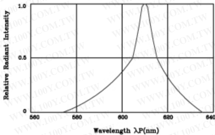
SPECTRAL DISTRIBUTION
