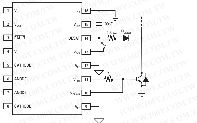
Figure 39. DESAT pin protection.
