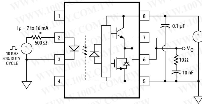
Figure 27. t_{PLH} , t_{PHL} , t_r , and t_f Test Circuit and Waveforms.
