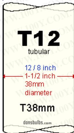
typical shape of T12 glass envelopes (not to scale)
