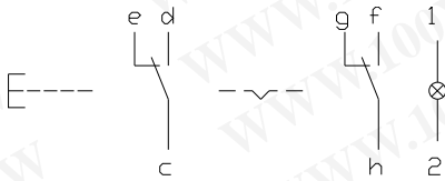
12 Illuminated pushbutton actuator page 8
