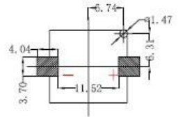
PCB Layout Diagram Top View
