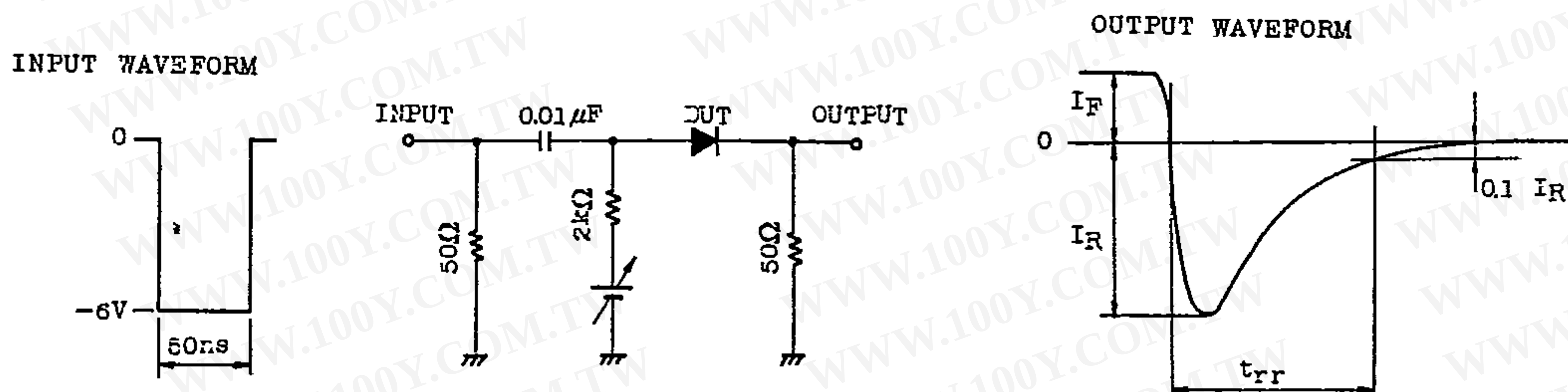
Fig. t_{rr} TEST CIRCUIT
