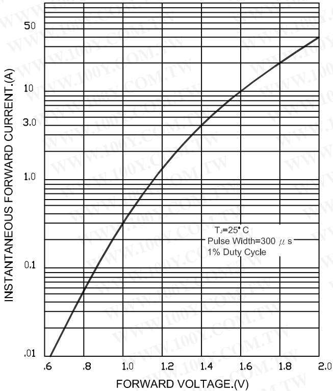
FIG.1-TYPICAL FORWARD CHARACTERISTICS
