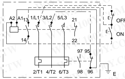
MS-N12, N20
