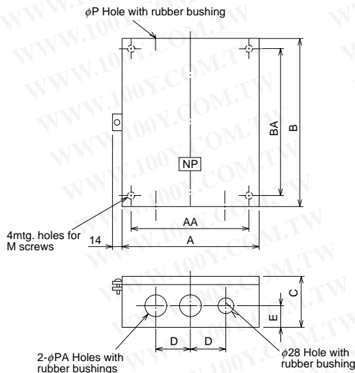
Type EYD-N20~N220
