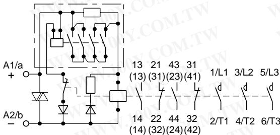
SD-N600, N800
