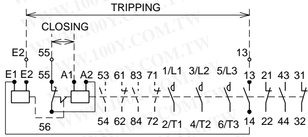
SHL-V□
